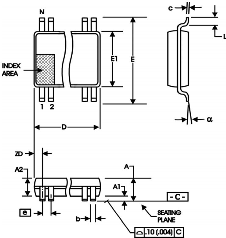
Package Outline - R Suffix for 28 Lead QSOP, 150MIL
