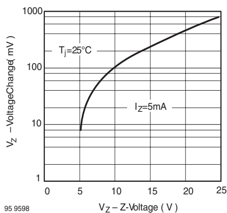
Figure 2. Typical Change of Working Voltage under Operating Conditions at T_{\text{amb}} = 25^\circ\text{C}
