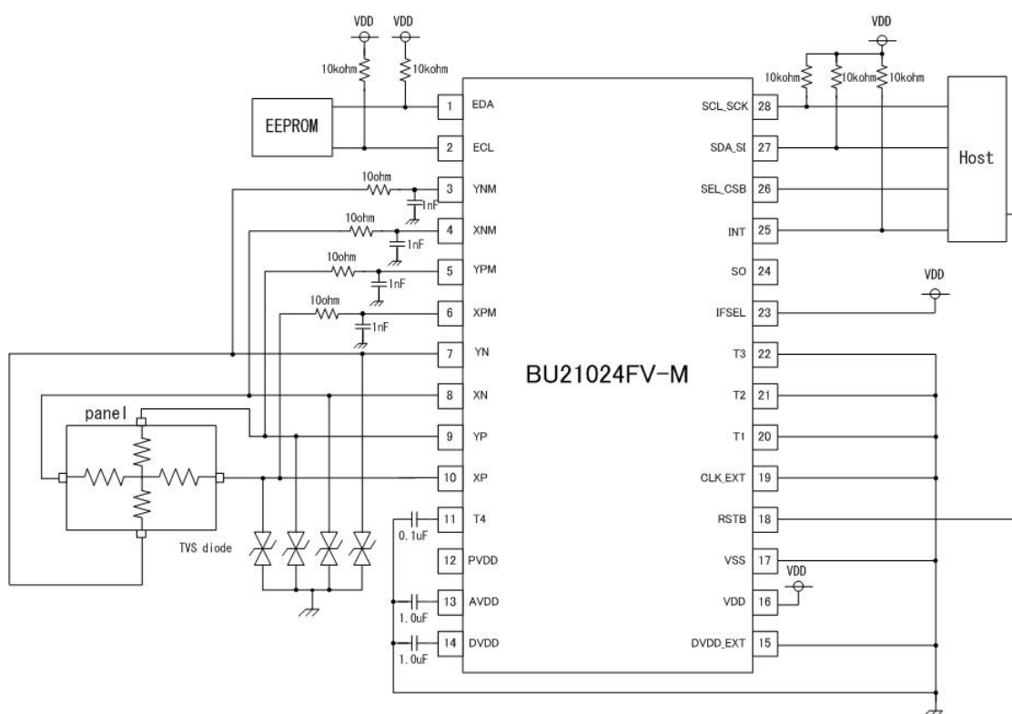
Example 6: BU21024FV-M Application Circuit (2-wire Serial bus with RC filter)
