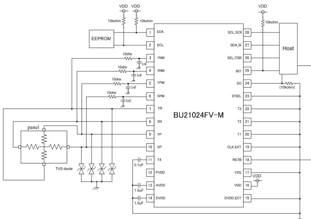
Example 5: BU21024FV-M Application Circuit (4-wireSPI with RC filter)
