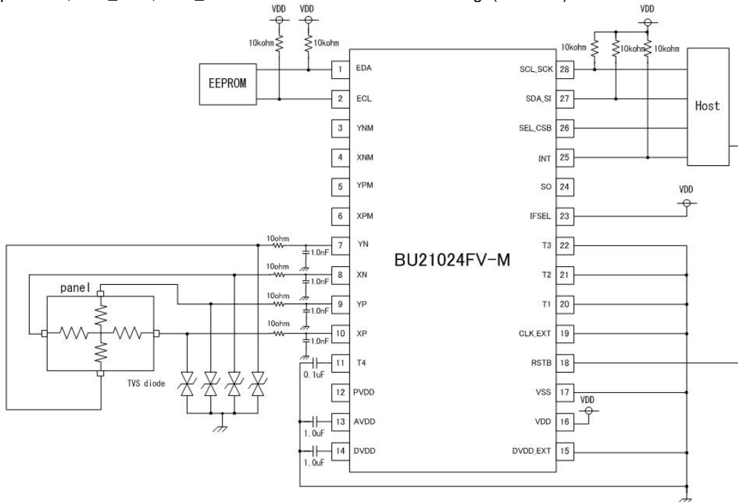
Example 4: BU21024FV-M Application Circuit (2-wire Serial bus)
