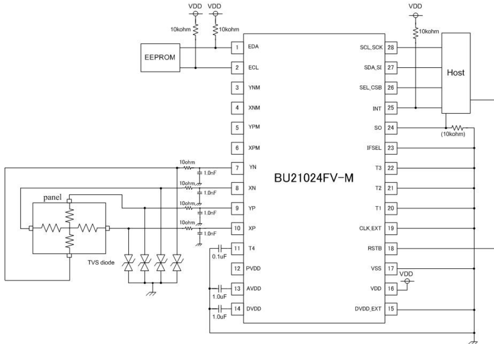
Example 3: BU21024FV-M Application Circuit (4-wireSPI)
