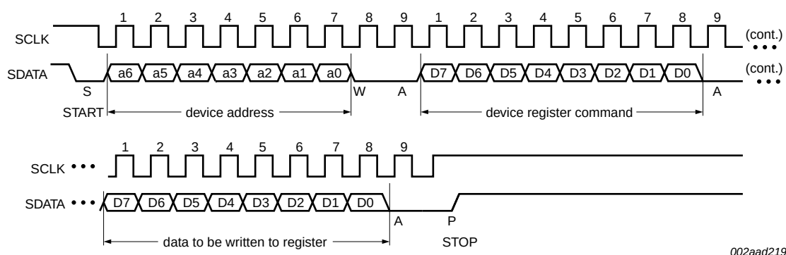
a. Write Byte format (to write a data byte to the device register)
