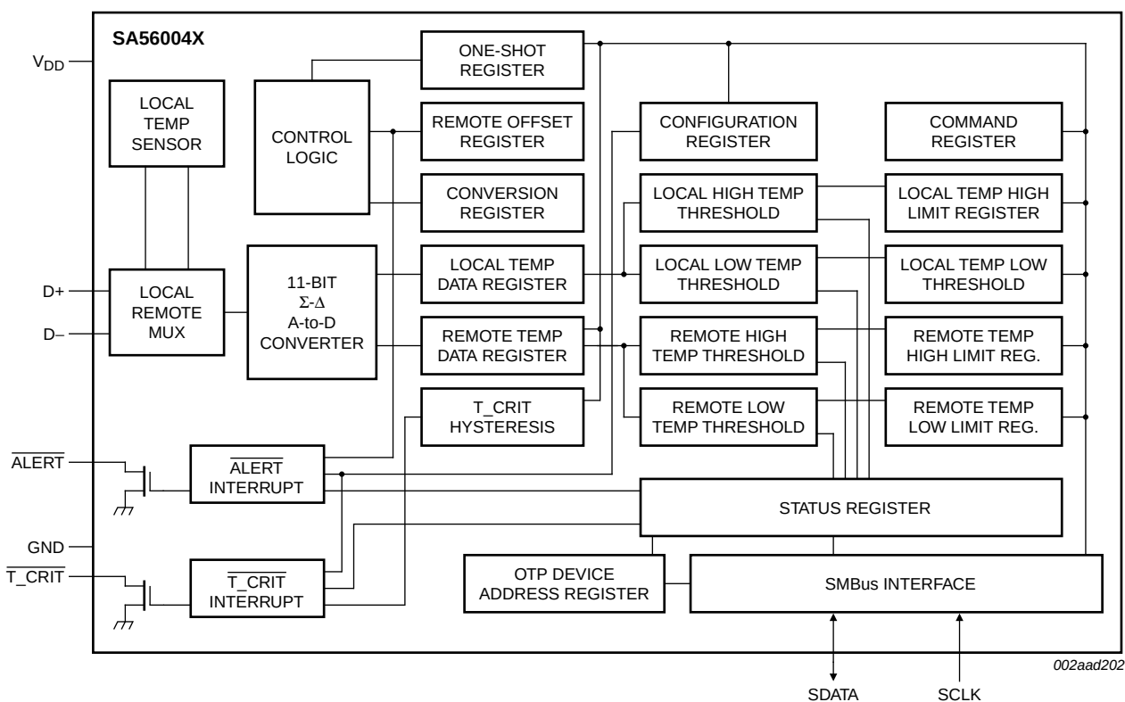
Fig 1. Block diagram
