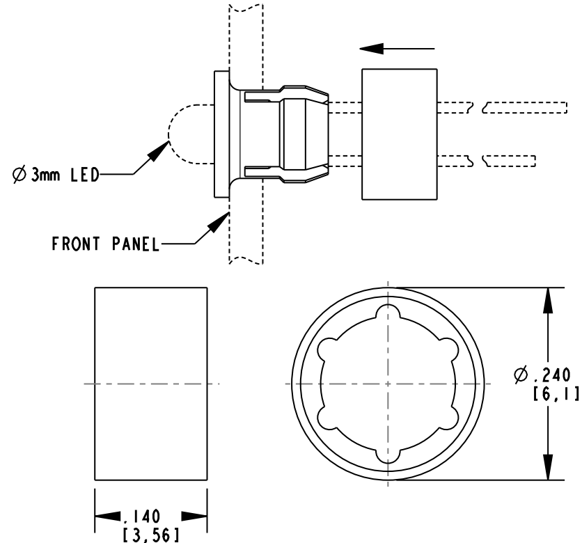
RETAINING RING
