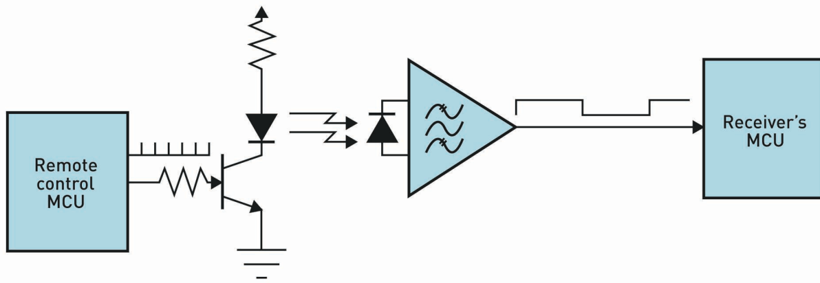
IR modulation and demodulation
