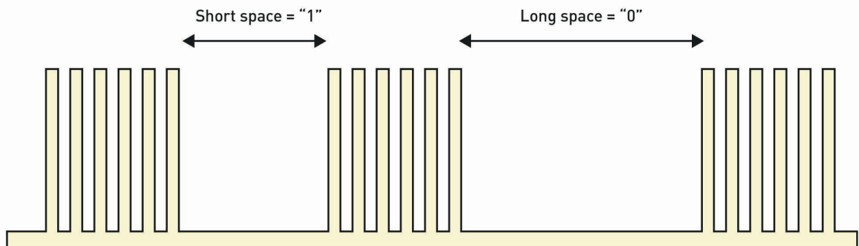
Pulse distance encoding
