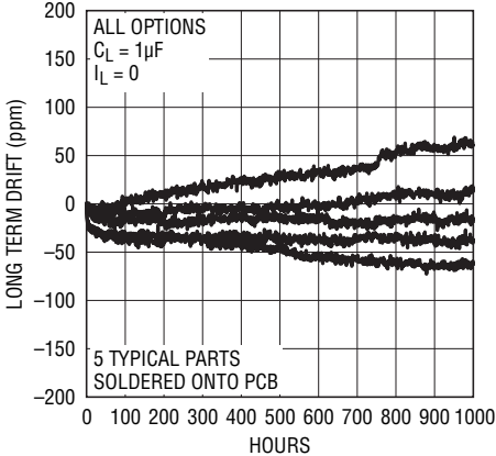
Long-Term Drift
