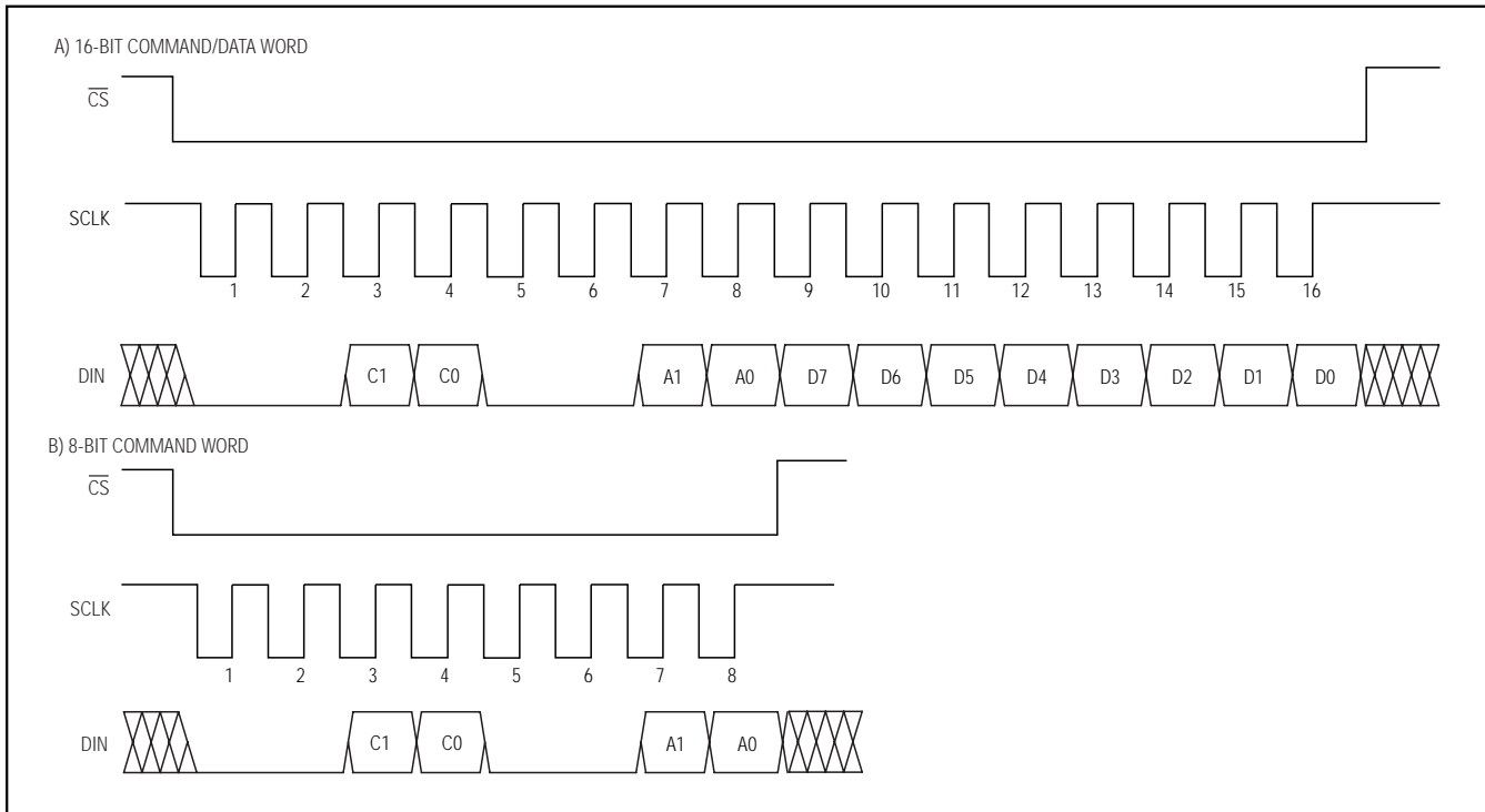
Figure 3. Digital-Interface Format
