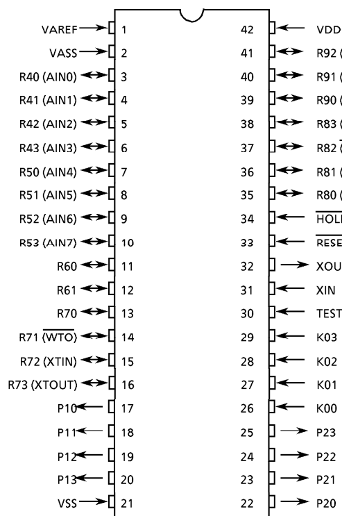
(1) SDIP42-P-600
