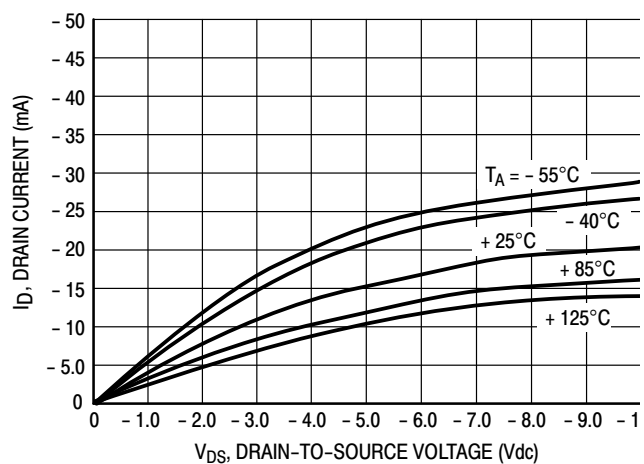
Figure 5. V_{GS} = -10 Vdc
