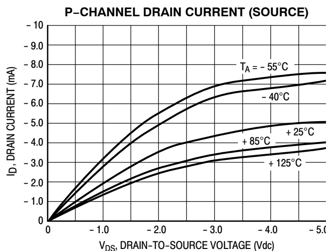
Figure 3. V_{GS} = -5.0 Vdc
