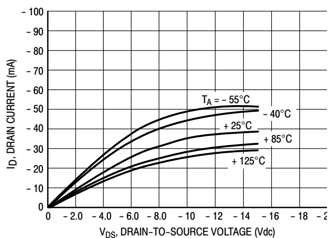
Figure 7. V_{GS} = -15 Vdc
