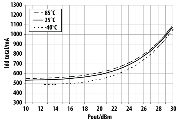
Figure 12. Over-temperature Idd_total vs Pout @ 2.5GHz
