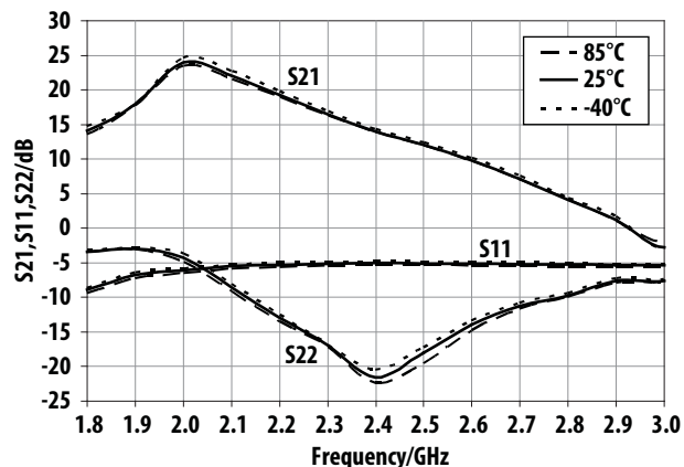
Figure 6. Small-signal performance in low-gain mode, V_{byp} = 5V
