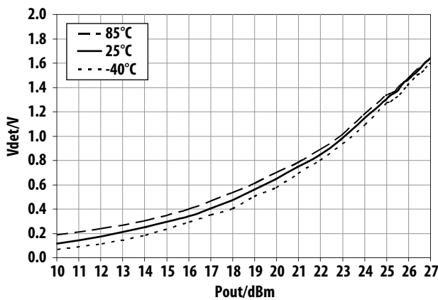
Figure 30. Over-temperature Vdet vs Pout @ 2.5GHz
