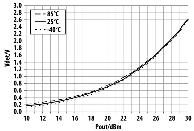
Figure 14. Over-temperature Vdet vs Pout @ 2.4GHz
