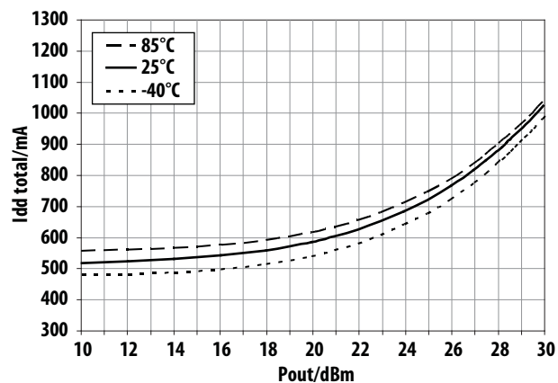
Figure 8. Over-temperature I_{dd\_total} vs P_{out} @ 2.3GHz
