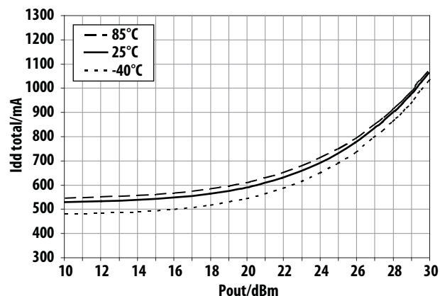
Figure 10. Over-temperature I_{dd\_total} vs P_{out} @ 2.4GHz
