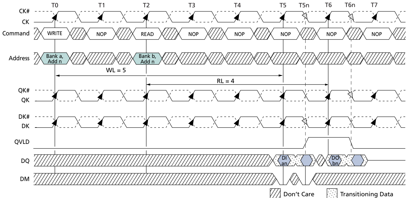
Figure 44: WRITE-to-READ
