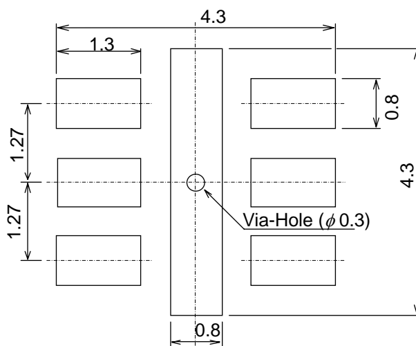
Fig.3 Desirable land area (in mm)
