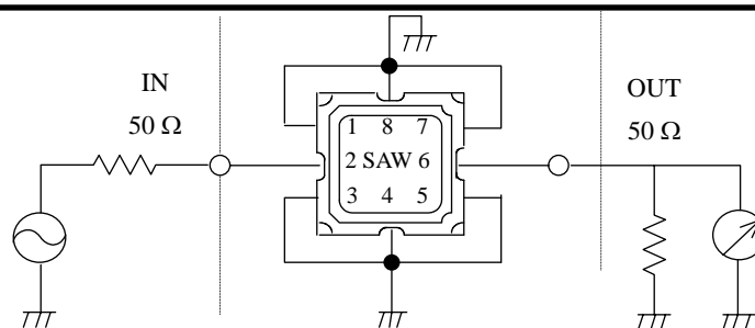
Fig.1 Measuring circuit
