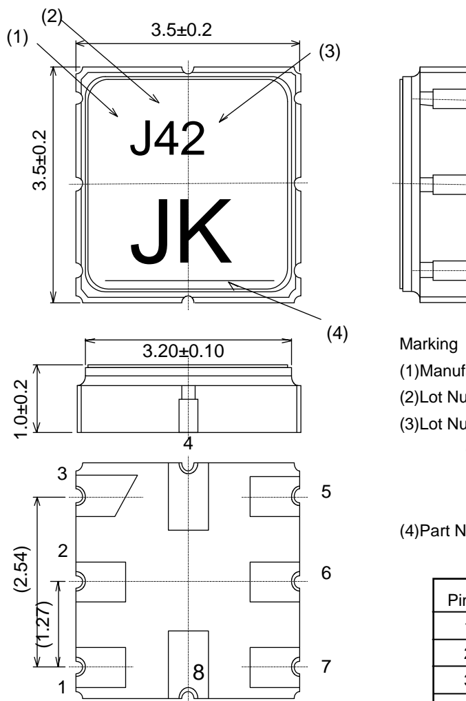
Fig.2 Package dimensions (in mm)
