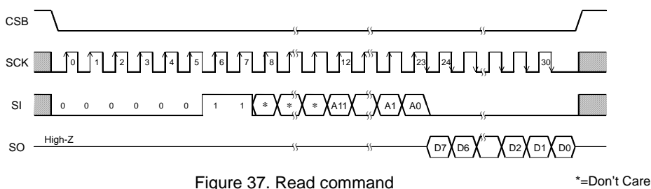
Figure 37. Read command
