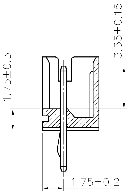
SECTION M-M
