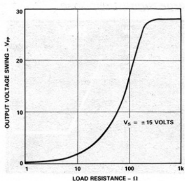
Figure 20. Output Voltage Swing vs. Load Resistance
