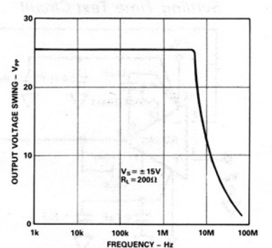
Figure 21. Large Signal Frequency Response
