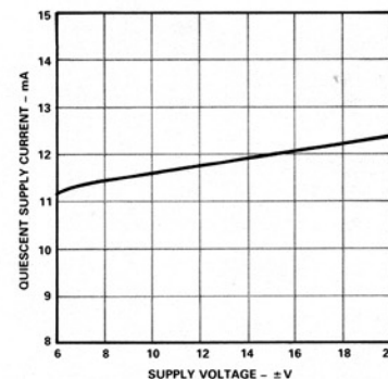
Figure 11. Supply Current vs. Supply Voltage
