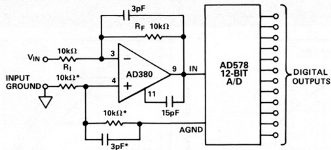
Figure 27. Fast-Settling Buffer
