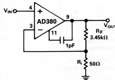
Figure 30. Video Amplifier
