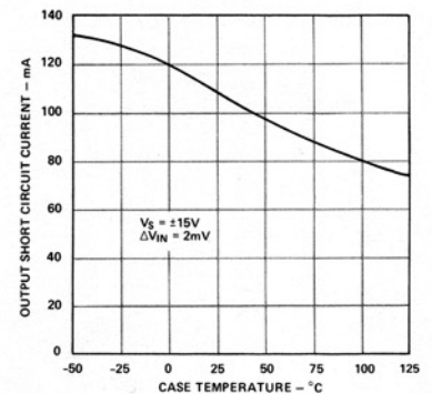
Figure 12. I_{SC} vs. Temperature
