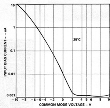
Figure 14. Input Bias Current vs. Common Mode Voltage
