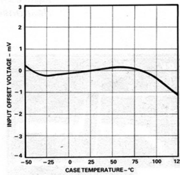
Figure 17. Offset Voltage vs. Temperature
