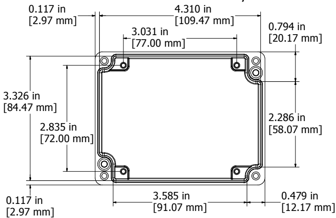
Top View Looking Inside Box
