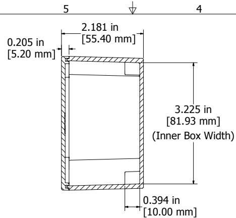
SECTION M-M End View of Assembly
