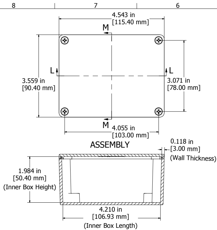
SECTION L-L Side View of Assembly
