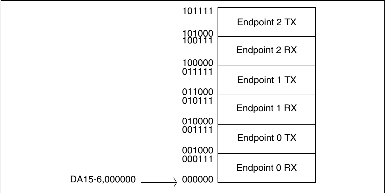
Figure 39. DMA Buffers
