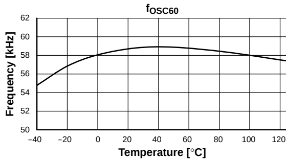
Figure 21. f_{\text{osc60}} vs. Temperature
