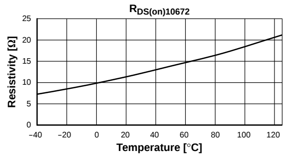
Figure 20. R_{\text{DS(on)10672}} vs. Temperature
