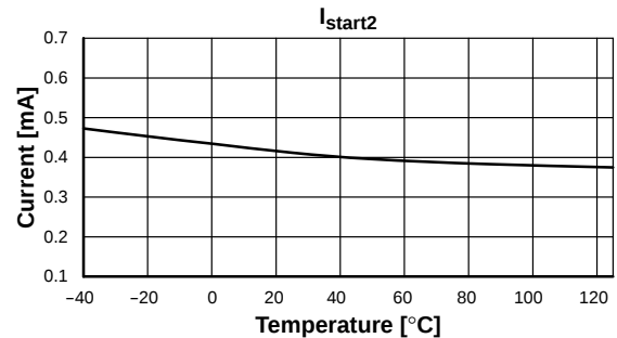
Figure 24. I_{\text{start2}} vs. Temperature
