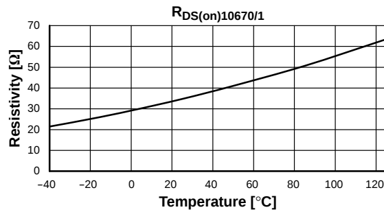
Figure 19. R_{\text{DS(on)10670/1}} vs. Temperature
