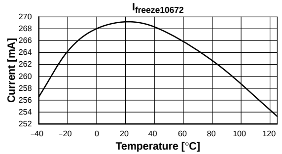
Figure 18. I_{\text{freeze10672}} vs. Temperature
