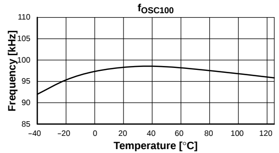
Figure 22. f_{\text{osc100}} vs. Temperature
