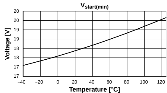
Figure 32. V start(min) vs. Temperature
