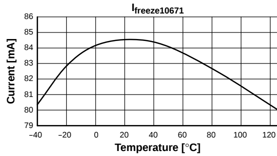
Figure 17. I_{\text{freeze10671}} vs. Temperature
