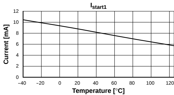
Figure 23. I_{\text{start1}} vs. Temperature
