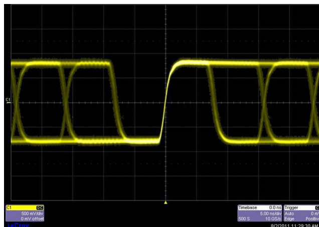
Figure 7. Receiver eye diagram
