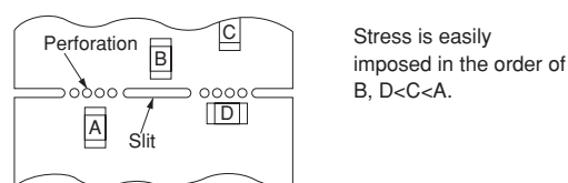
[Chip Mounting Close to Board Separation Point]
