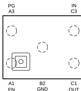
Pin Functions
