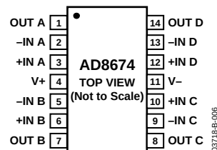
Figure 6. 14-Lead TSSOP (RU Suffix)
