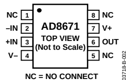
Figure 2. 8-Lead MSOP (RM Suffix)
