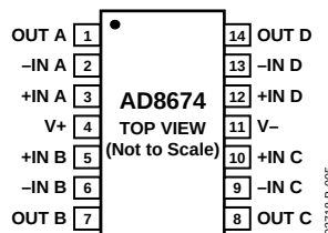
Figure 5. 14-Lead SOIC (R Suffix)
