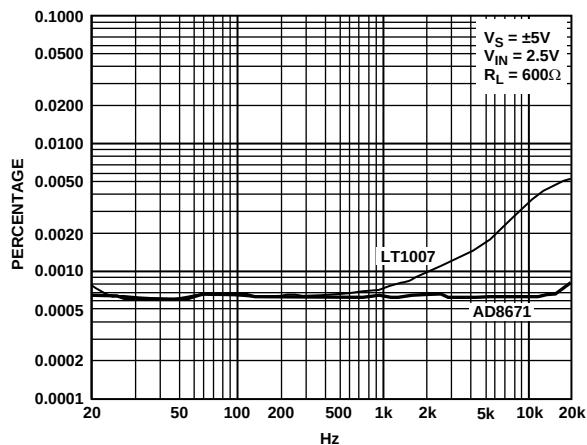
Figure 35. Total Harmonic Noise and Distortion
