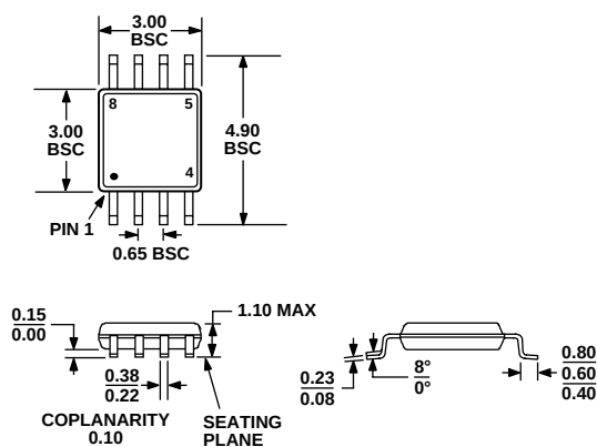
Figure 44. 8-Lead Micro Small Outline Package [MSOP] (RM-8) Dimensions shown in millimeters
