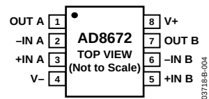
Figure 4. 8-Lead MSOP (RM Suffix)
