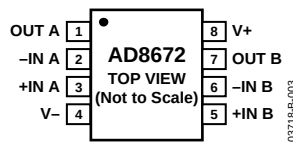
Figure 3. 8-Lead SOIC (R Suffix)
