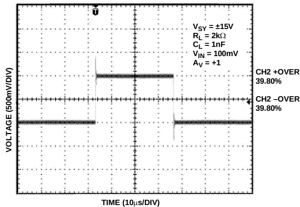
Figure 36. Capacitive Load Drive
