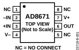
Figure 1. 8-Lead SOIC (R Suffix)
