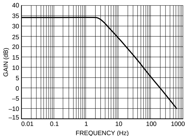
Figure 41. Forward Gain Plot
