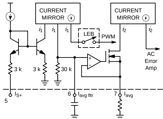
Figure 32. Current Sense Amplifier
