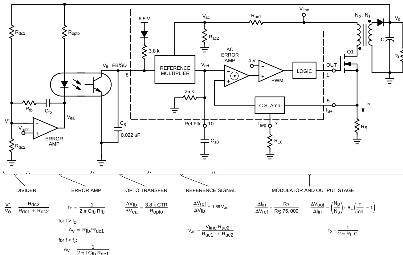
Figure 39. Voltage Regulation Loop
