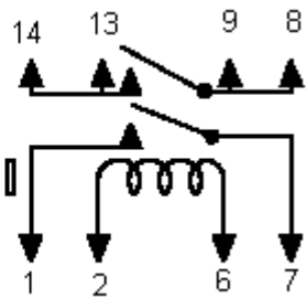
Figure E DPST-NO without diode
