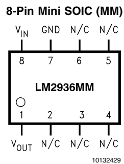
Top View Order Number LM2936MM-3.3 See NS Package Number MUA08A
