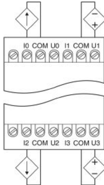
Connection diagram
