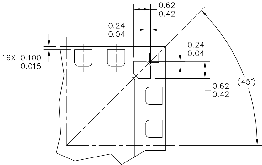
DETAIL M
