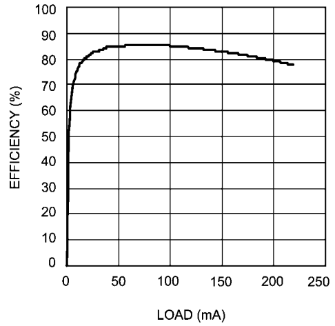
Efficiency vs Load Current - "Y" V_{IN} = 3.3V, V_{OUT} = 12V
