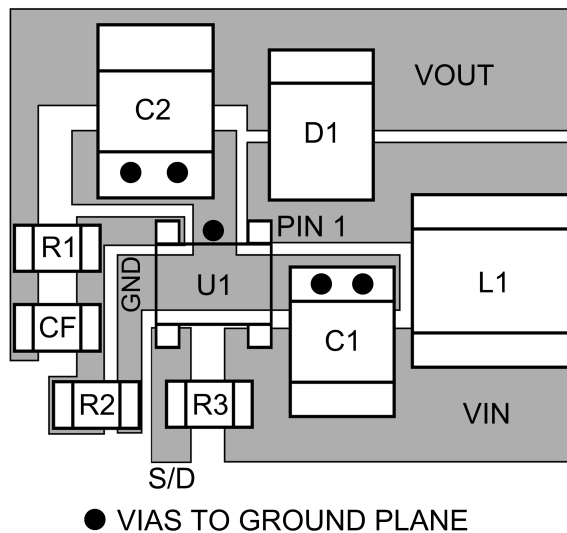
Recommended PCB Component Layout
