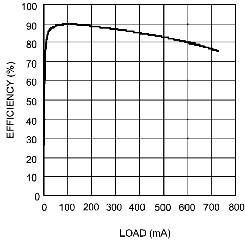
Efficiency vs Load Current - "Y" V_{IN} = 3.3V, V_{OUT} = 5V
