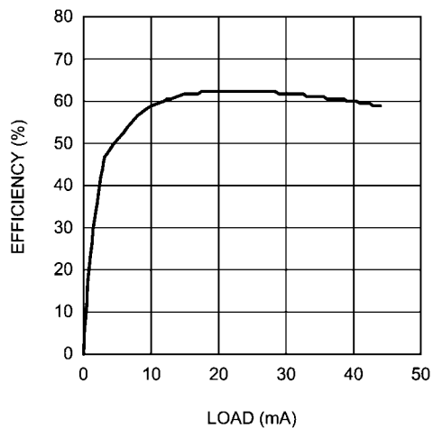
Efficiency vs Load Current - "X" V_{IN} = 2.7V , V_{OUT} = 12V
