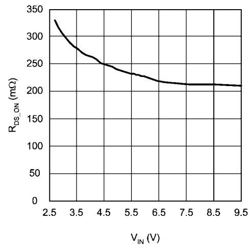
R_{DS(ON)} vs V_{IN}
