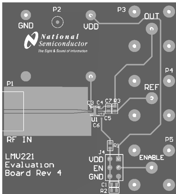
Figure 1. LMV221 Evaluation Board
