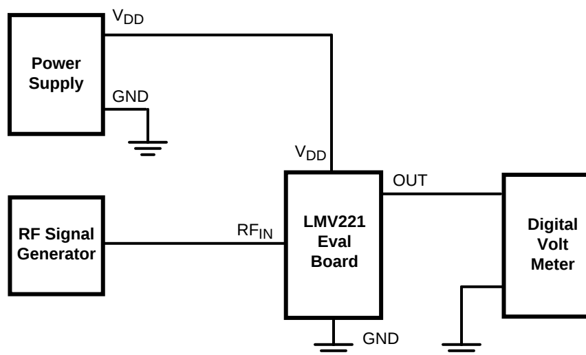
Figure 5. Measurement Setup
