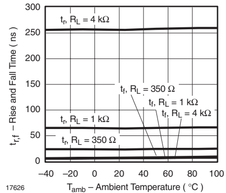
Figure 21. Rise and Fall Time vs. Ambient Temperature
