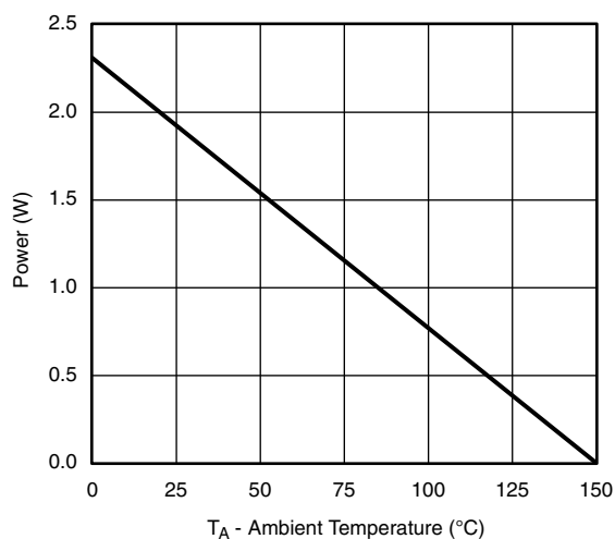
Power, Junction-to-Ambient
