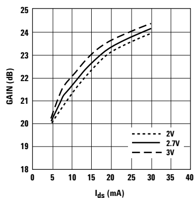
Figure 16. Gain vs. I_{ds} and V_{ds} at 900 MHz. [1]
