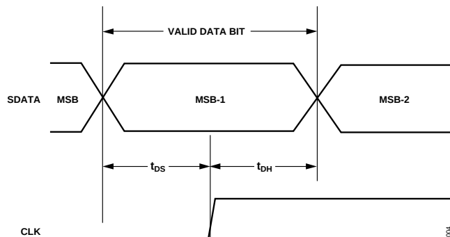
Figure 4. SDATA Timing
