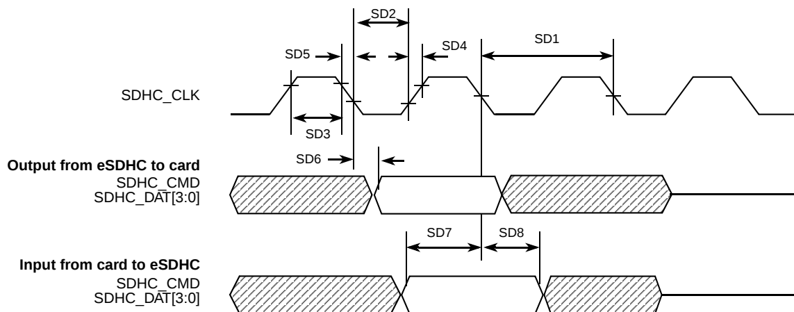
Figure 29. eSDHC Timing
