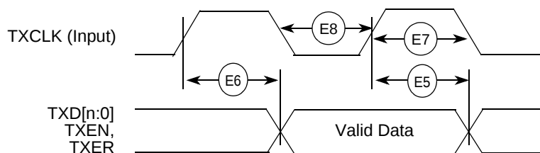
Figure 24. MII Transmit Signal Timing Diagram
