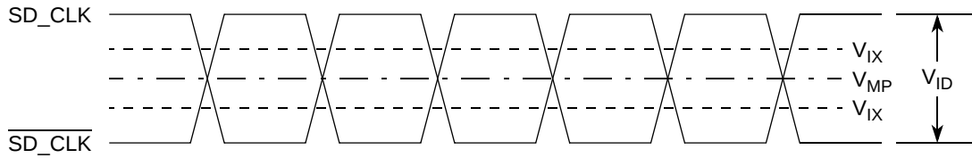
Figure 15. \text{SD\_CLK} and \overline{\text{SD\_CLK}} Crossover Timing
