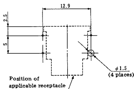
HR12-10R-SP(71)(Stopper plate) (Applicable PCB thickness range 1~2)
