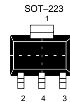
TOP VIEW See Mech. Drawings Section
