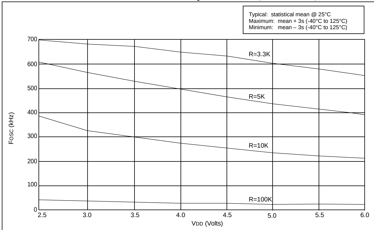
FIGURE 16-4: TYPICAL RC OSCILLATOR FREQUENCY vs. V_{DD} , C_{EXT} = 300\text{ pF} , 25^{\circ}\text{C}
