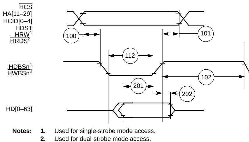
Figure 15. Asynchronous Broadcast Write Timing Diagram
