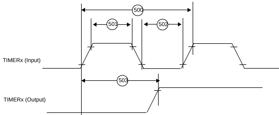
Figure 21. Timer Timing
