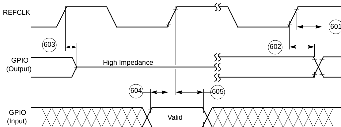
Figure 26. GPIO Timing
