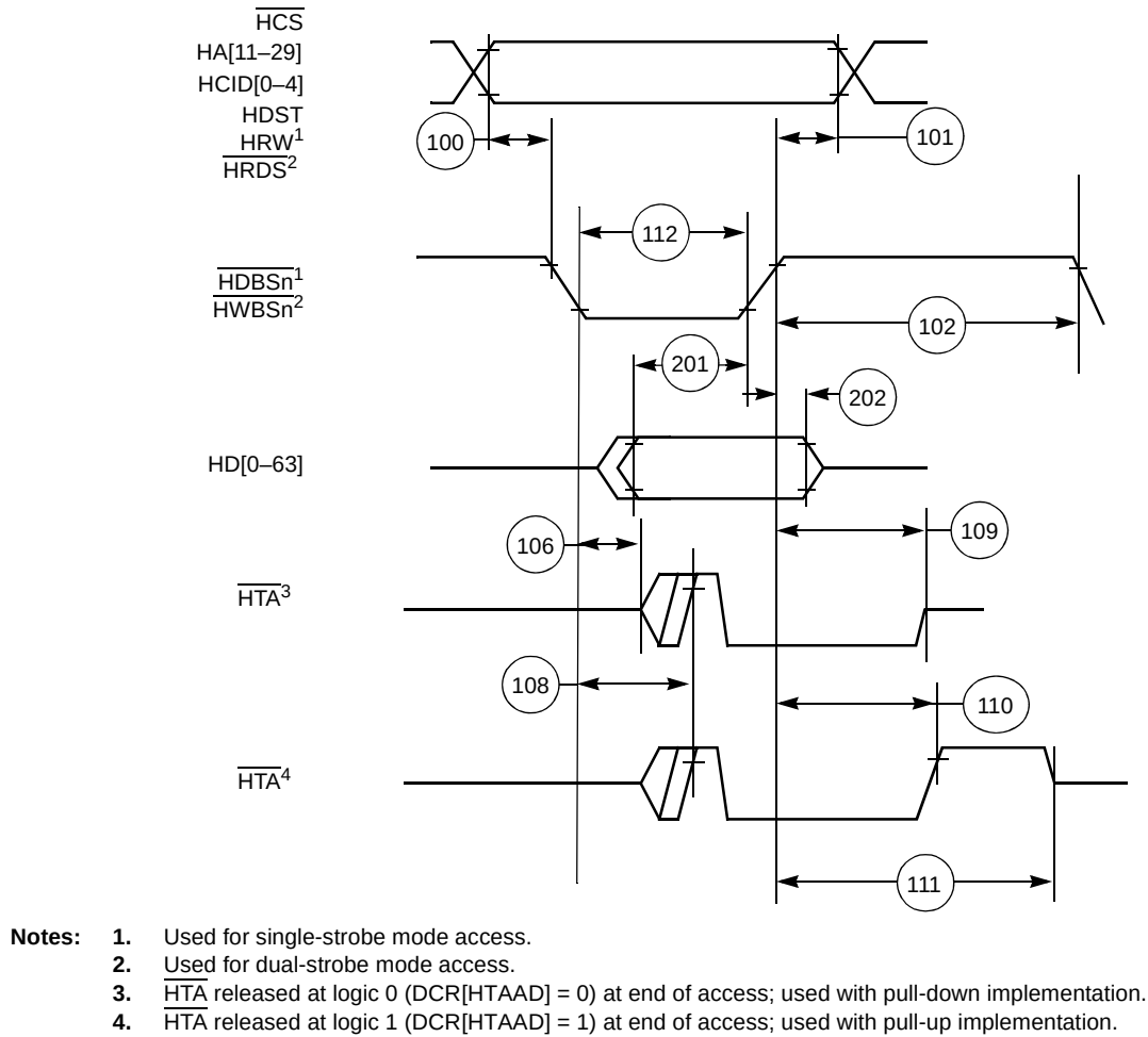
Figure 14. Asynchronous Single- and Dual-Strobe Modes Write Timing Diagram
