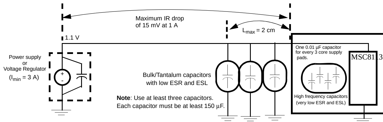
Figure 32. Core Power Supply Decoupling
