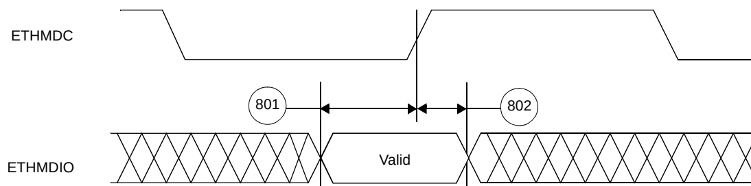
Figure 22. MDIO Timing Relationship to MDC
