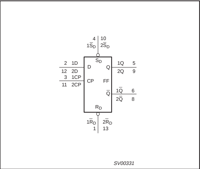
LOGIC SYMBOL
