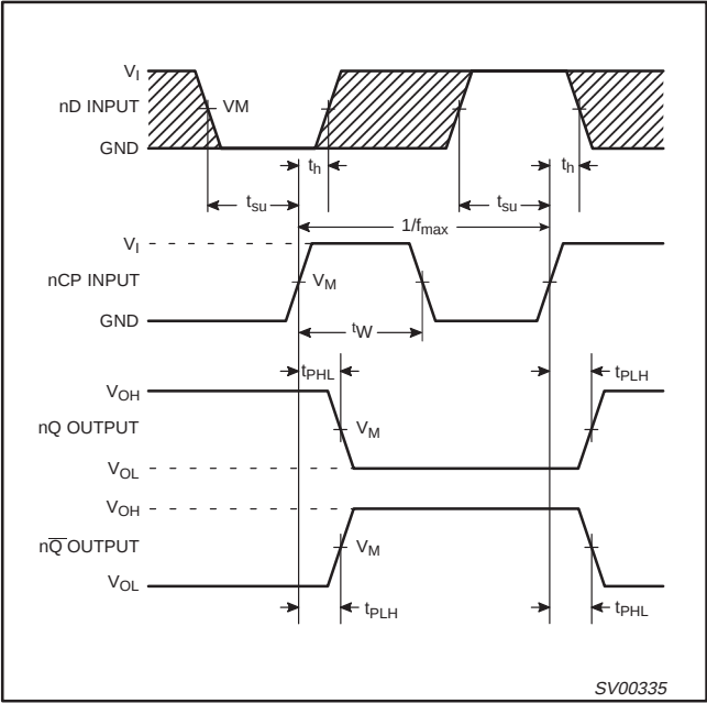
Figure 1.The clock (nCP) to output (nQ, nQ) propagation delays, the clock pulse width, the nD to nCP setup times, the nCP to nD hold times, the output transition times and the maximum clock pulse frequency
