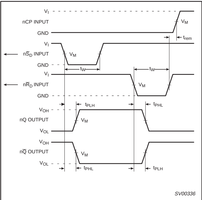
Figure 2.The set ( n\bar{S}_D ) and reset ( n\bar{R}_D ) input to output (nQ, nQ) propagation delays, the set and reset pulse widths and the n\bar{R}_D to nCP removal time
