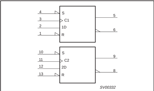
LOGIC SYMBOL (IEEE/IEC)
