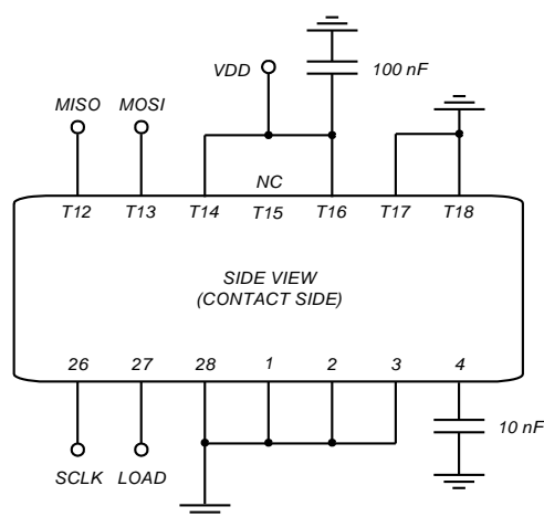
Figure 9-2 SAR100 electrical connections (vertical mount)
