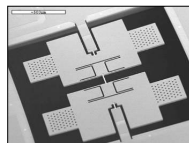
Figure 1-1: SAR100 element structure
