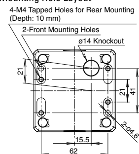
Mounting Hole Layout
