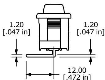
"R" TERMINAL
