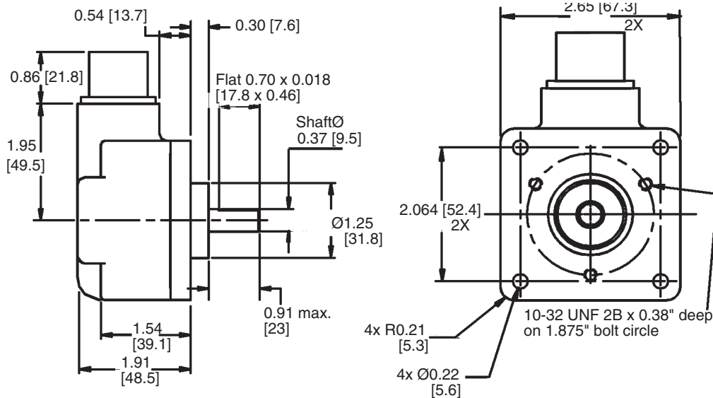
Standard Housing
