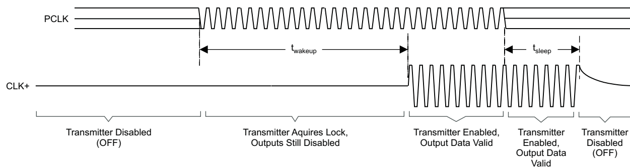
Figure 14. Standby Detection
