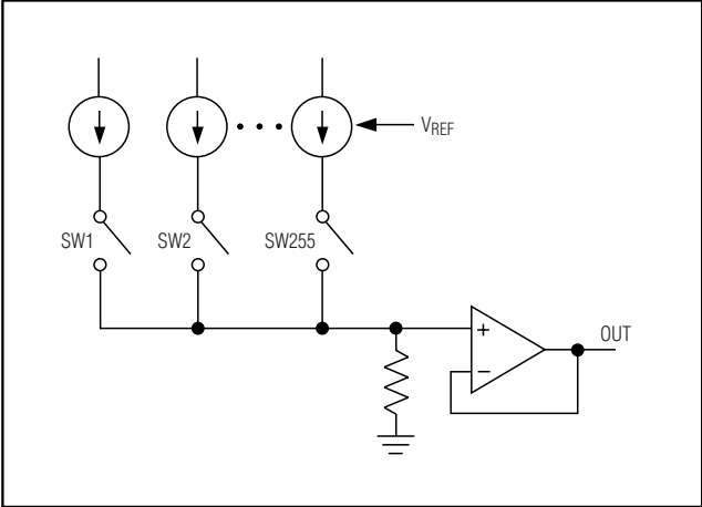
Figure 2. Current-Steering Topology
