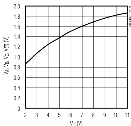
LOGIC-LEVEL THRESHOLD vs. V_+
