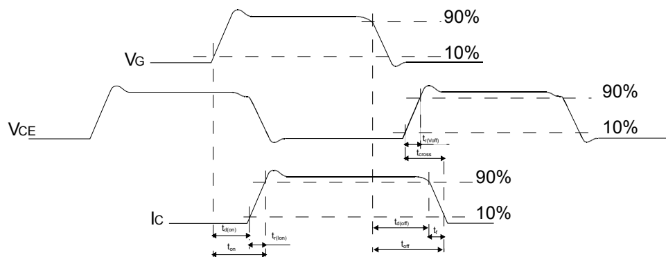
Figure 28. Switching waveform
