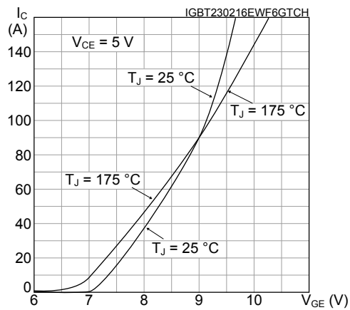
Figure 13. Transfer characteristics
