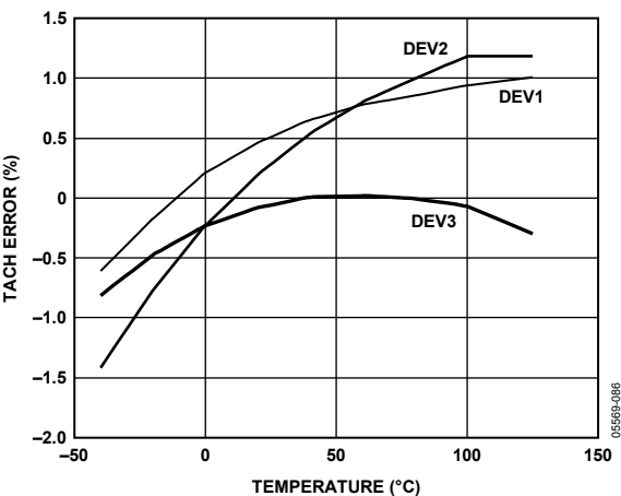
Figure 24. TACH Accuracy vs. Temperature
