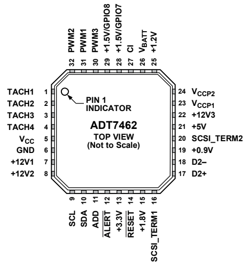
Figure 6. Configuration Option 3
