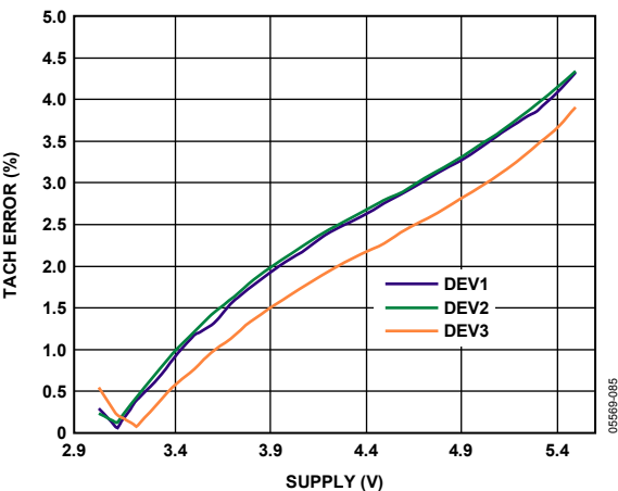
Figure 23. TACH Accuracy vs. Supply Voltage
