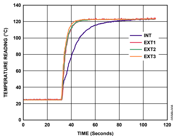
Figure 14. DUT Response to Thermal Shock
