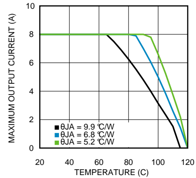
Figure 54. Thermal Derating Curve
